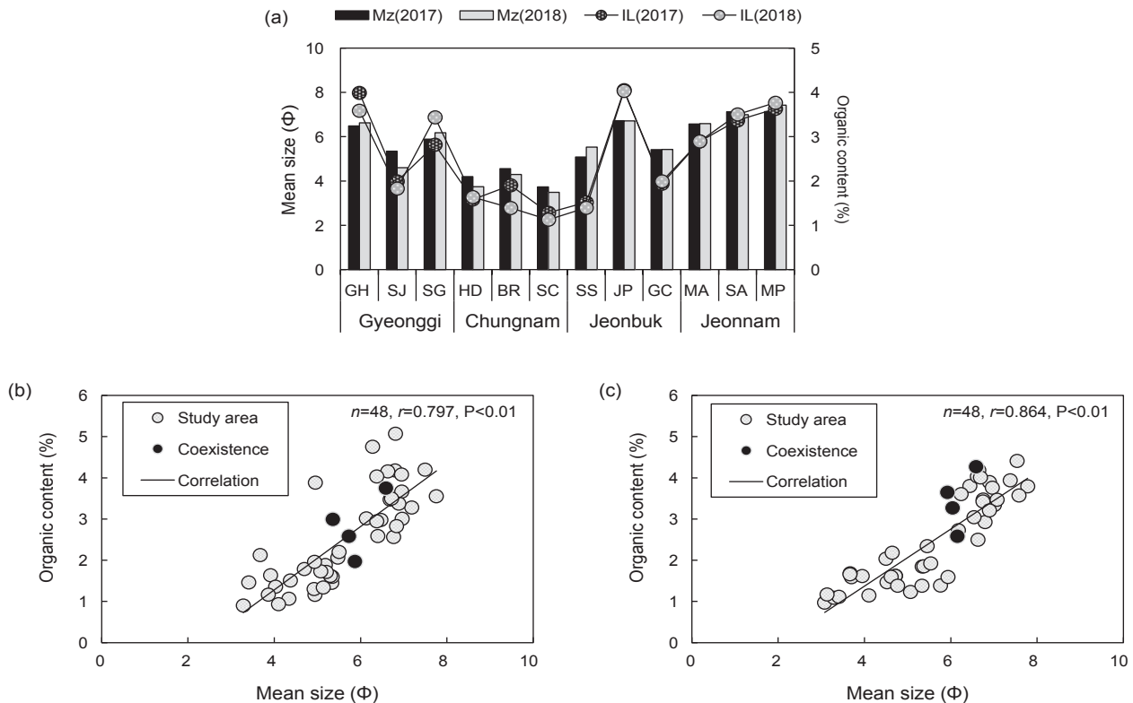
Fig. 3. Relationships between sediment mean size and organic content (ignition loss). Organic content versus mean size: (b) 2017, (c) 2018. r is the correlation, n is the number of samples, and P is the statistical P value.
